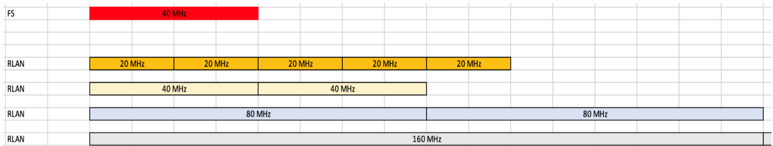
Figure 12: WAS/RLAN Channelization
