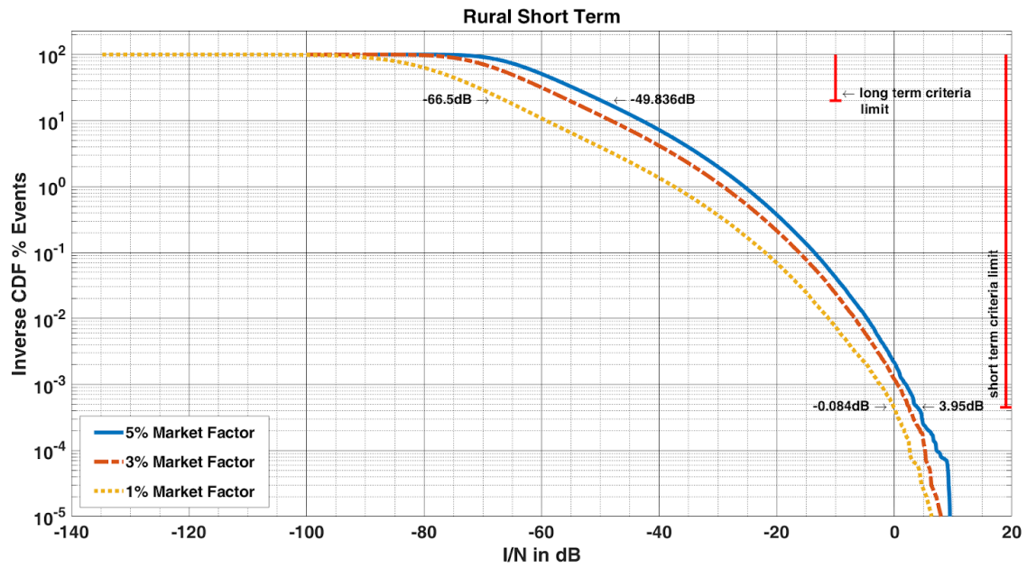
Figure 19: Short-term Scenario Rural at FS Height of 48m and at different Market adoption factors
