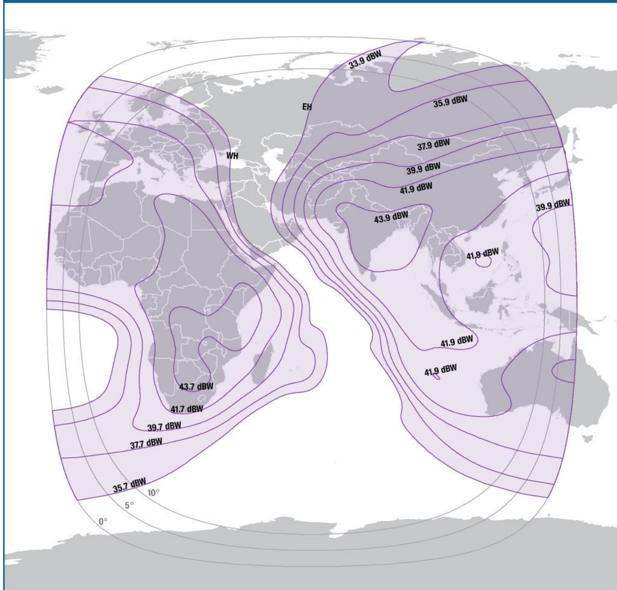
Figure 20: Intelsat 39 Footprint
