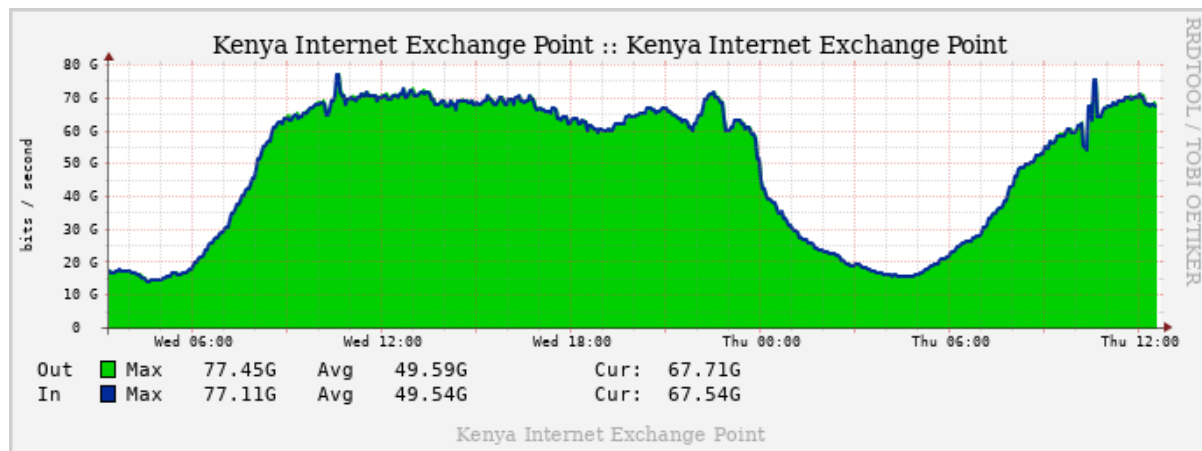
Figure 11: Image of Data throughput profile in Kenya as at 8th-9th September 2022
