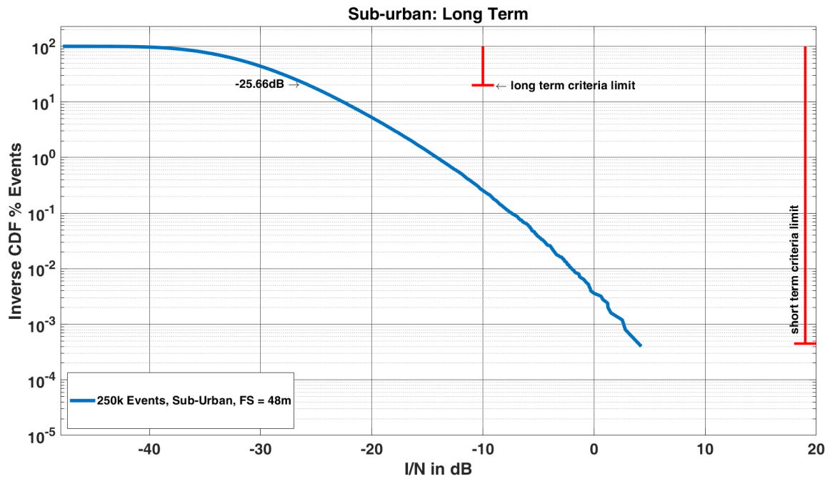
Figure 15: Long-term Scenario Suburban at FS Height of 48m
