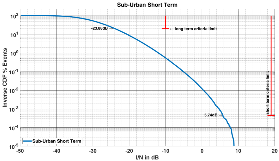
Figure 18: Short-term Scenario Sub-Urban at FS Height of 48m
