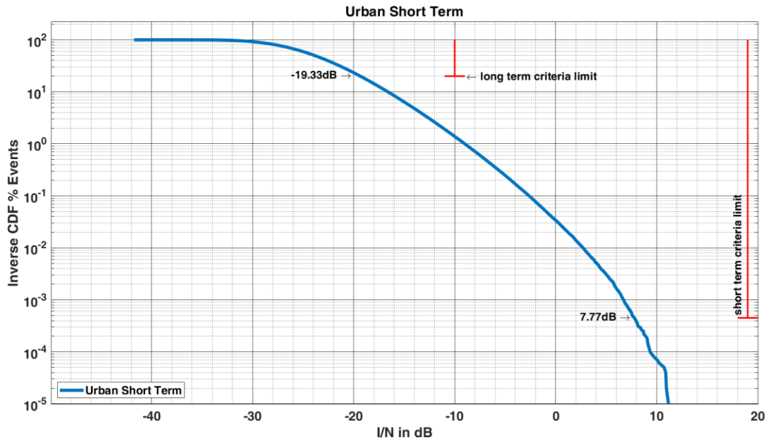
Figure 17: Short-term Scenario Nairobi at FS Height of 48m
