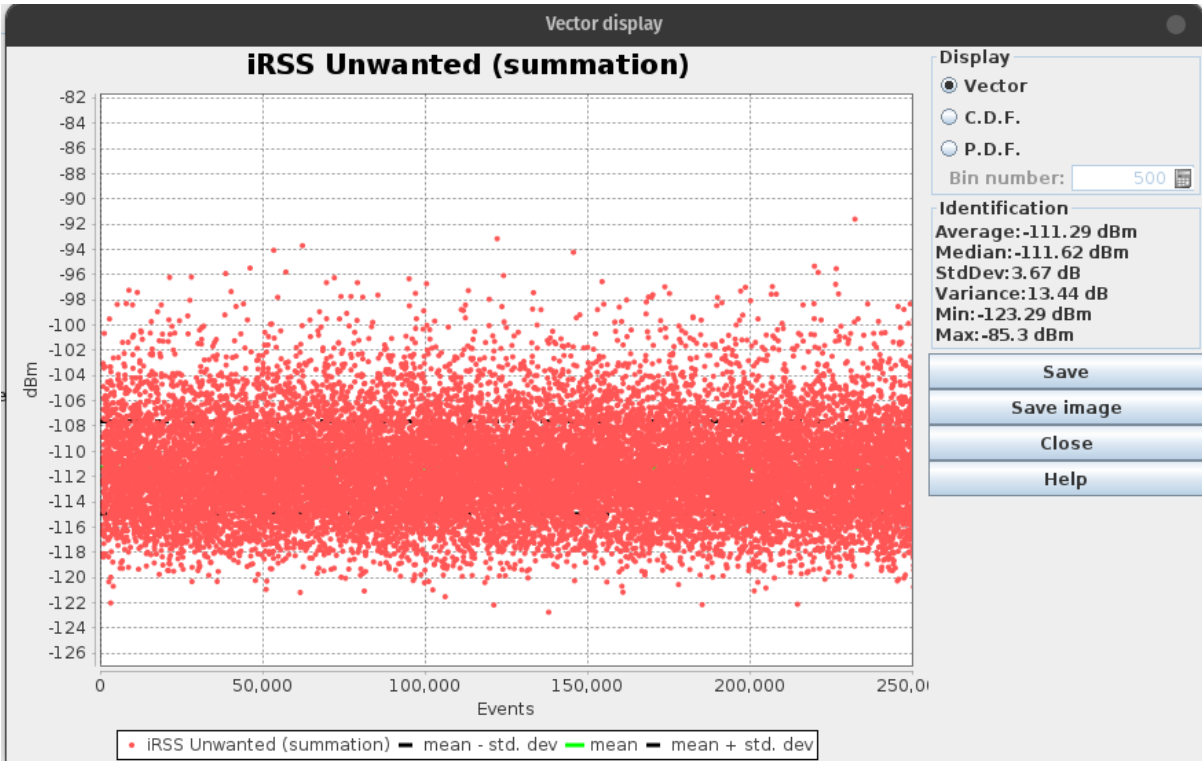
Figure 9: SEAMCAT Screenshot of the iRSS Unwanted generated from the simulation events for a long-term scenario
