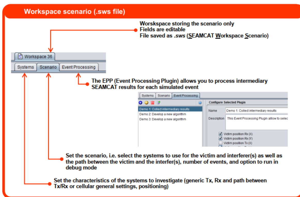
Figure 3: SEAMCAT interface showing a simulation instance of a Workspace
