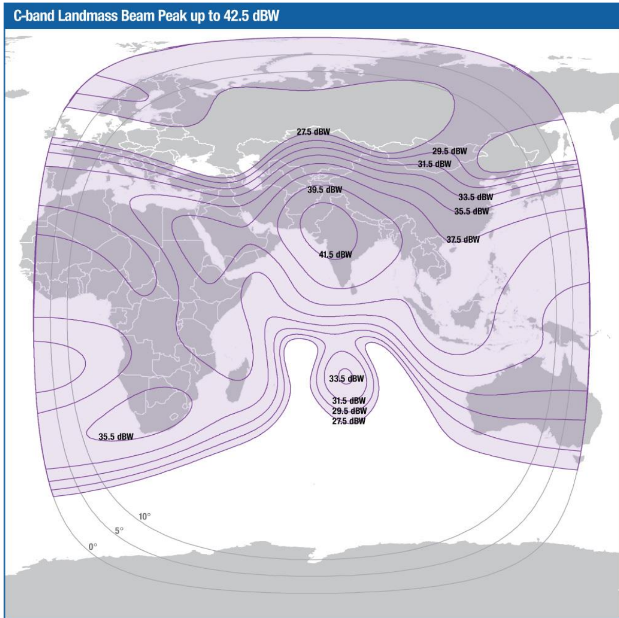
Figure 23: Intelsat 36 Footprint
