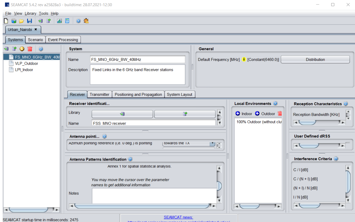
Figure 2: SEAMCAT Tool Interface - version 5.4.2
