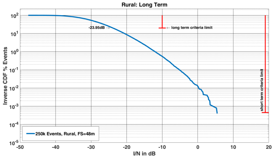
Figure 16: Long-term Scenario Rural at FS Height of 48m
