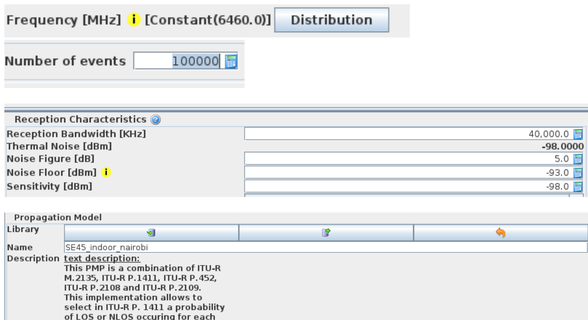
Figure 6: SEAMCAT screenshots on Frequency, No. of Events, Reception Characteristics and Propagation Model
