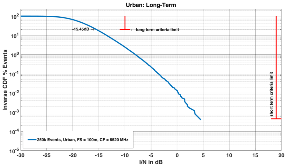
Figure 14: Long-term Scenario Urban at an FS Height of 100m
