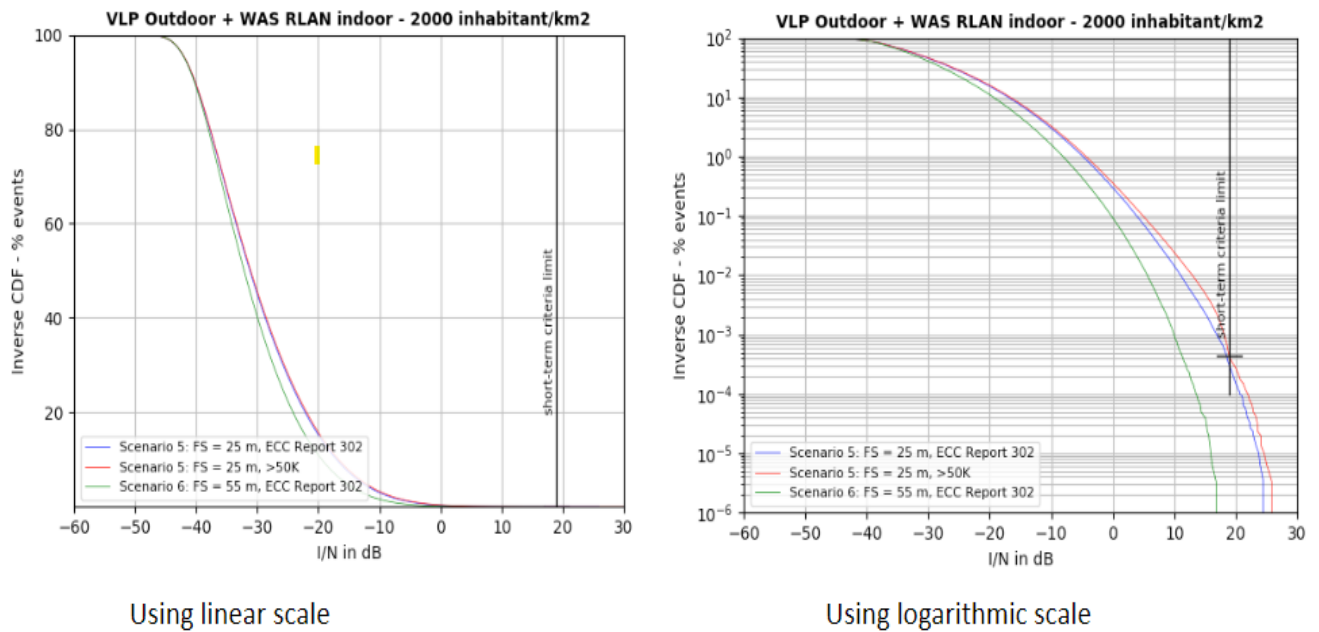
Figure 13: Two output graphs of a simulation with linear and logarithmic abscissa scales
