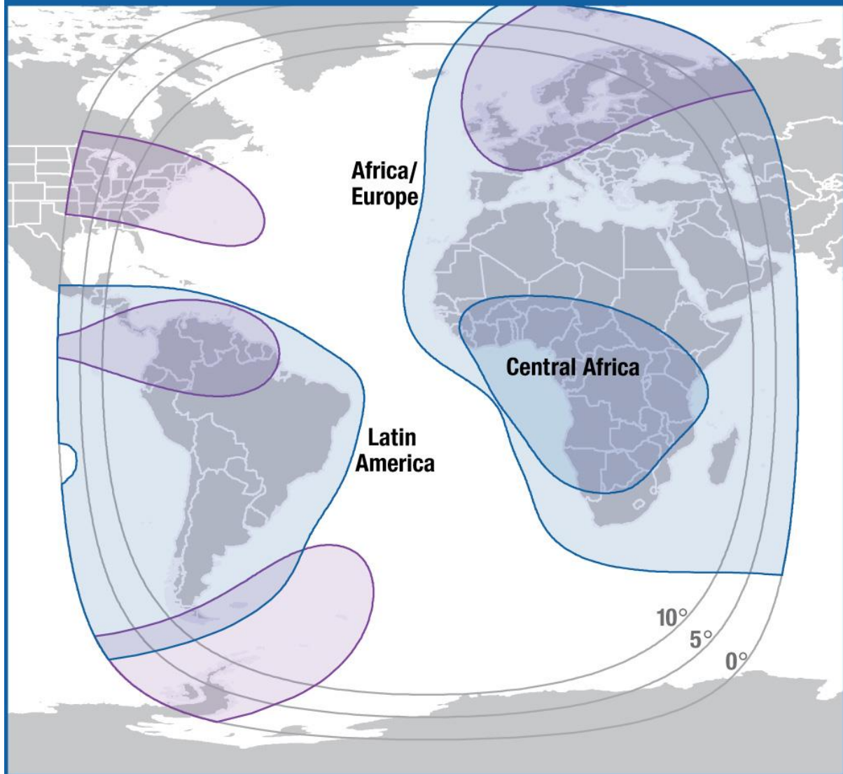
Figure 21: Intelsat 37E Footprint
